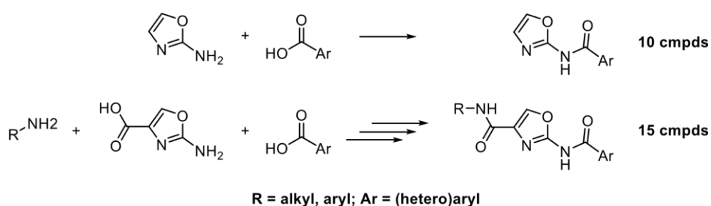
Figure 1. Synthetic diagram and general structures of the investigated derivatives
