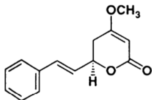
Kawain
