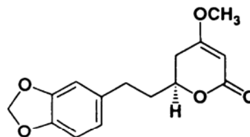
Dihydromethysticin
